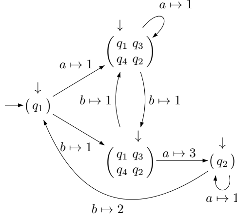
FIGURE 4. Construction of the Mealy automaton from the two-tape DFA of FIGURE 1(B)
