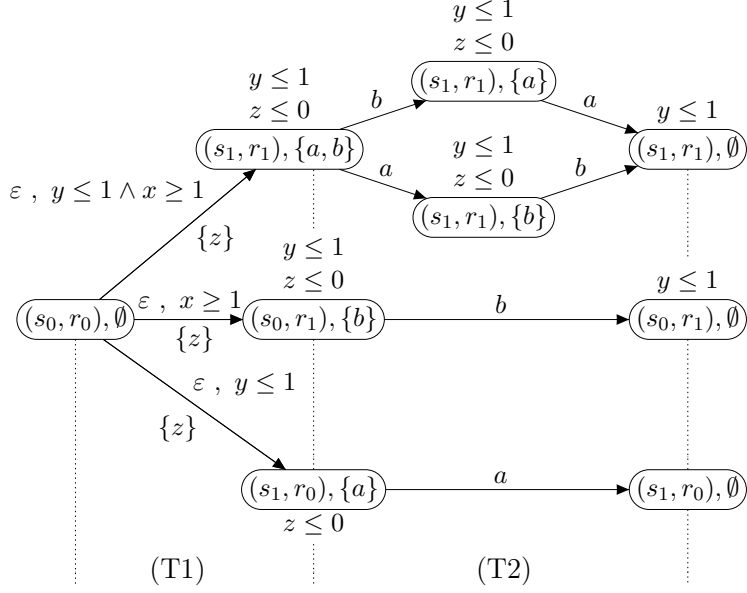
Figure 4: Part of the icTA \mathcal{B}_{\mathcal{D}} for the DTA \mathcal{D} from Figure 1
