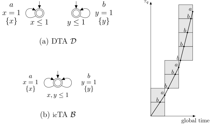
Figure 5: An example of “weird” behaviour
