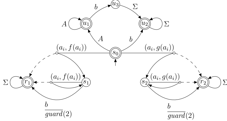
Figure 11: Encoding of PCP: icTA \tilde{\mathcal{B}}
