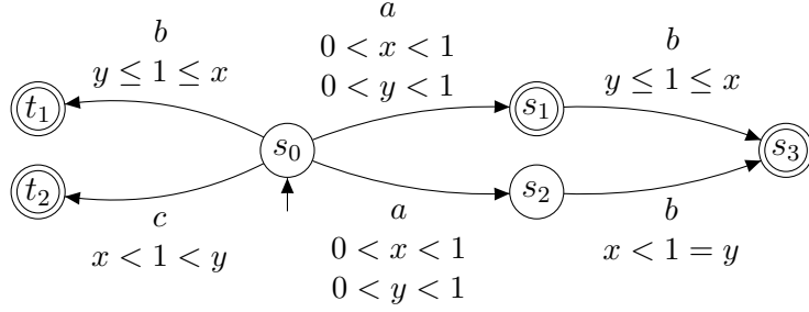
Figure 3: An icTA \mathcal{B} with independent clocks x and y
