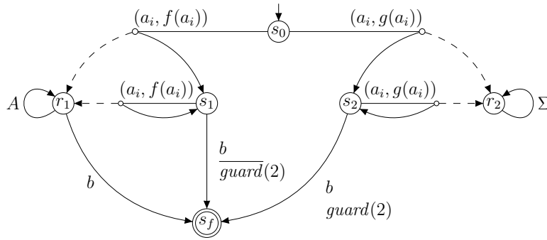
Figure 9: Encoding of PCP: icTA \mathcal{B}
