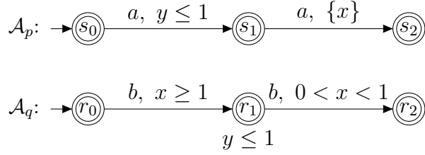
Figure 1: A distributed timed automaton over \{p, q\}
