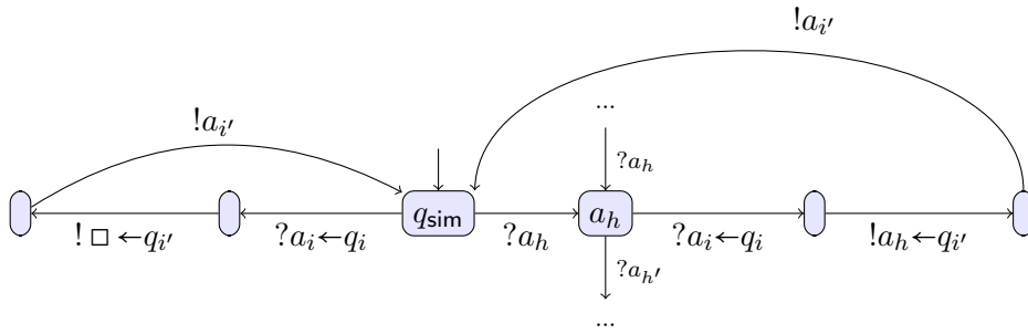
Figure 3.4: Encoding of a transition of \mathfrak{M} moving the head to the left.
