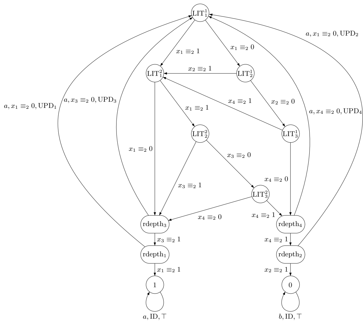
Fig. 6. ESSA associated with \forall x_1 \exists x_2 \forall x_3 \exists x_4 (x_1 \vee x_2 \vee x_4) \wedge (\neg x_1 \vee x_3 \vee \neg x_4)
