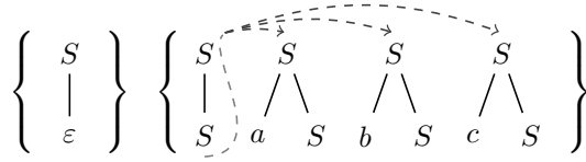
Figure 4: An UVG-dl for L_{\text{mix}} .
