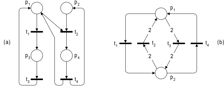
Fig. 1. Examples of II-nets
