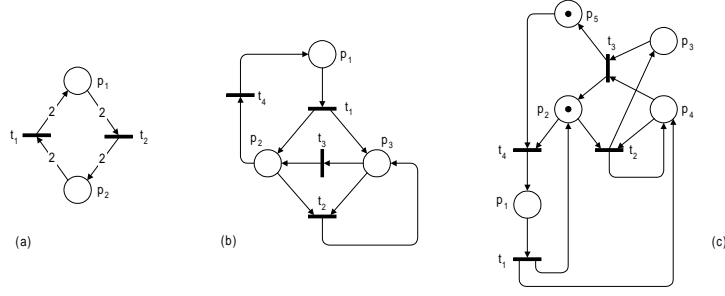
Fig. 4. \Pi -net and potential reachability: (a) \text{PRS}(\mathbf{m}_0) \neq \text{PRS}^{\text{B}}(\mathbf{m}_0) , unbounded (b) and bounded (c) \Pi -systems with spurious marking
