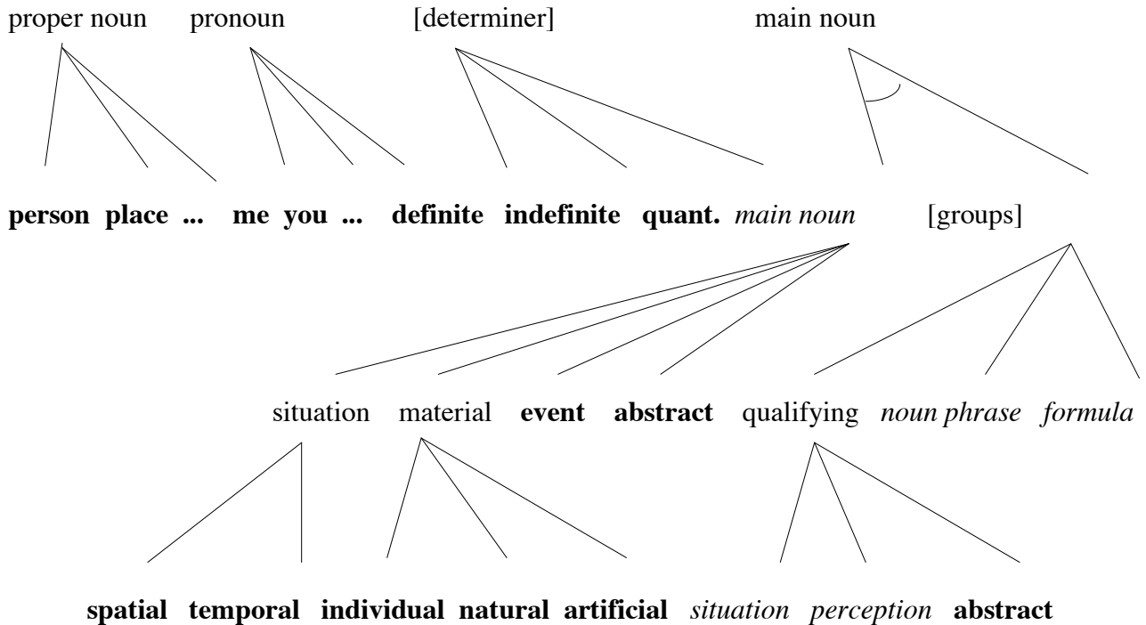
Fig. 2. And/or tree of the substituable morphemes taken into account in noun phrases.
