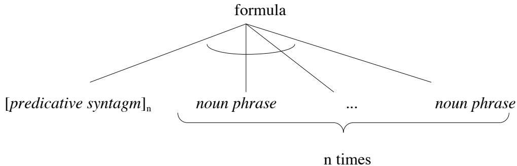
Fig. 3. And/or tree giving the structure of propositions.
