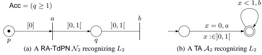
Fig. 2. A language L_2 not recognized by any 0-reset integral RA-TdPN
